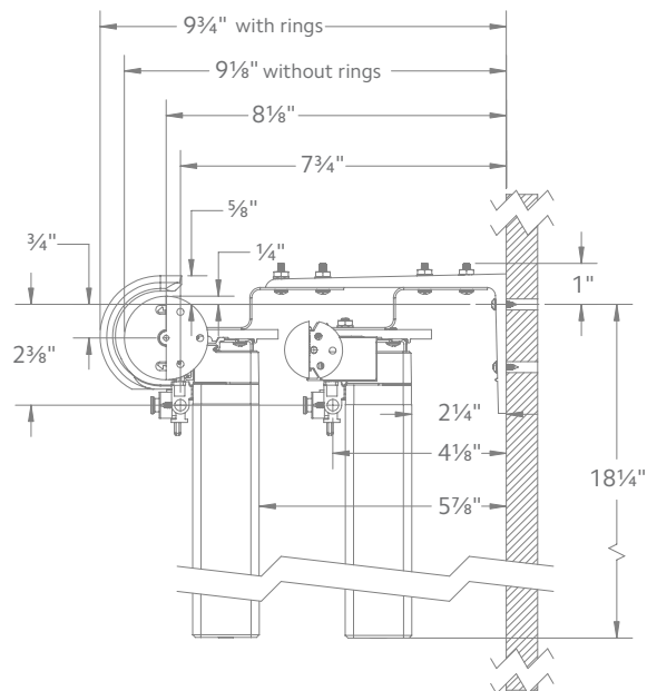
2" & 1 3/8" DOUBLE MOUNT
